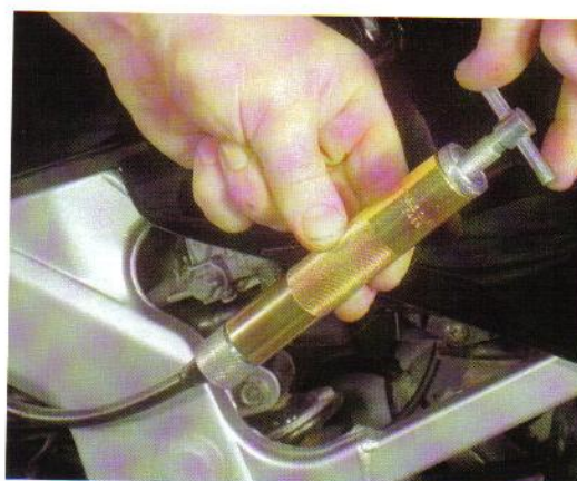
Pressure lubricator forces light oil in between the cable inner and outer
