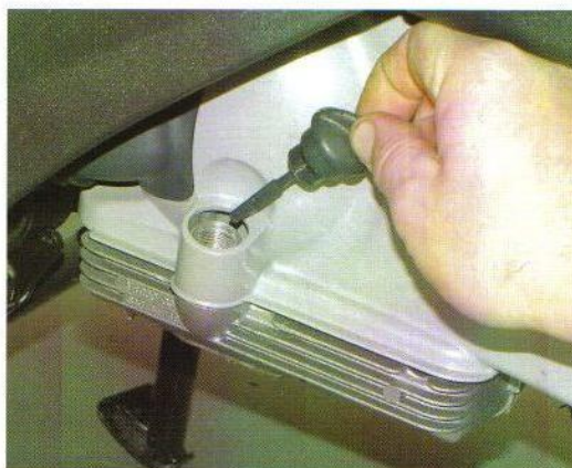
Remove filler cap/dipstick to facilitate quicker draining of used engine oil. Leave it somewhere prominent to remind you to refill the sump before riding off!
