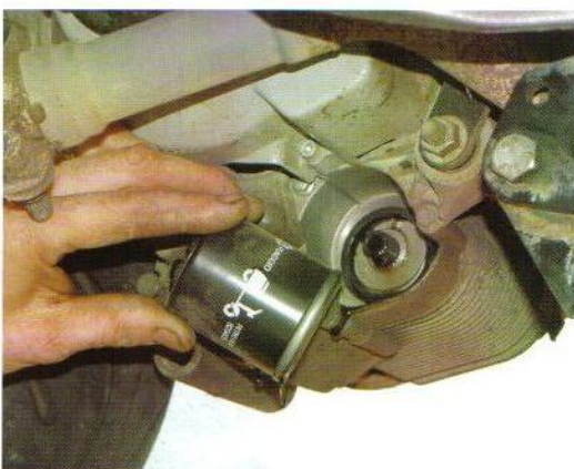
Disposable oil filter elements such as these cannot be cleaned out and should be replaced at the recommended intervals. Sometimes at every oil change, otherwise every other oil change
