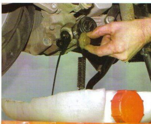
A cut-down oil container or similar makes a useful and cheap reusable drain tray. Oil is best drained when warm, but take care not to scald yourself
