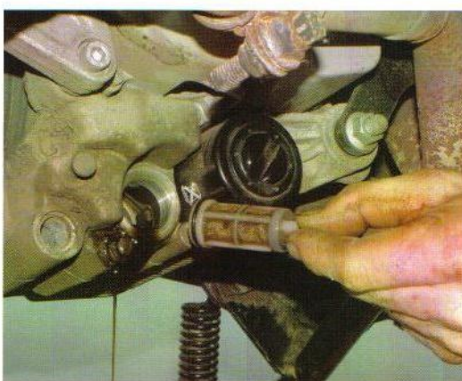
Gauze filters should be removed, inspected and cleaned and refitted provided they are in good condition, if not they must be replaced
